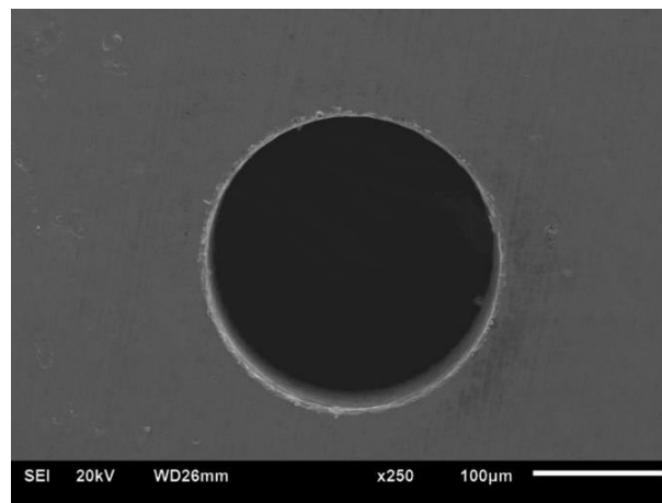
Micro hole fabricated using micro-EDM
