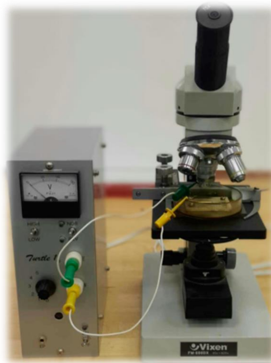
Micro Electric Discharge Machine
